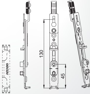
Alt Kilitleme-1, 420-950
