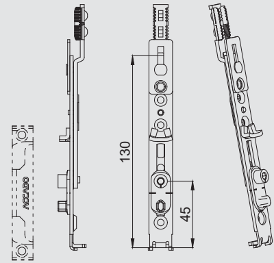
Alt Kilitleme-2, 950-2350
