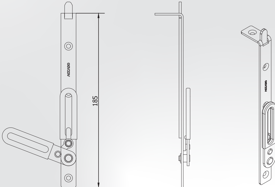
Shoot Bolt with Lever Top/Bottom 185 mm
