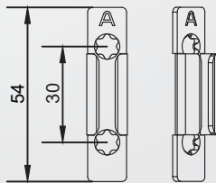
Sliding Gear Locking Plate - Steel
