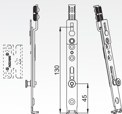
Extension Piece Se, 90°
