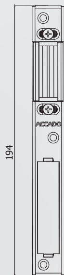
Adjustable Door Locking Plate Eco With Deadbolt Box
