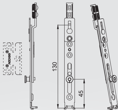
Extension Piece Se, 180°
