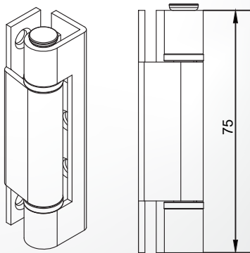
Steel Hinge, 75 mm
