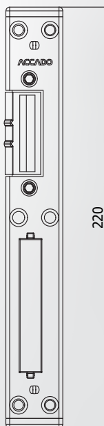
Adjustable Door Locking Plate With Deadbolt Box
