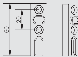
Sliding Gear Locking Plate - Zamak
