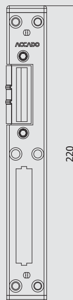
Adjustable Door Locking Plate Without Deadbolt Box
