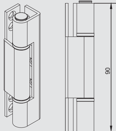
Steel Hinge, 90 mm
