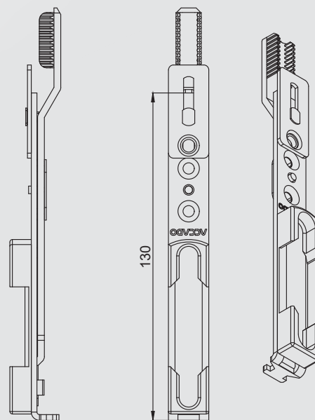
Shoot Bolt, Bottom
