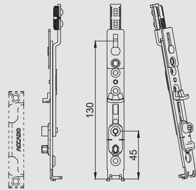
Bottom Extension-2, 950-2350
