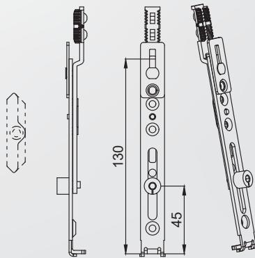
Extension Piece, 180°
