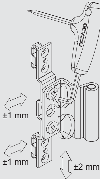
Middle Hinge Adjustment
