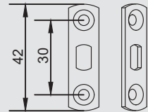
Sliding Gear Centering Piece
