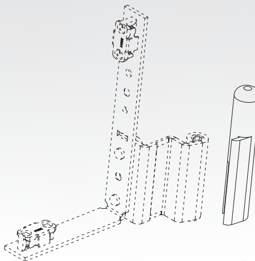
Adjustable Bottom Hinge Cover
