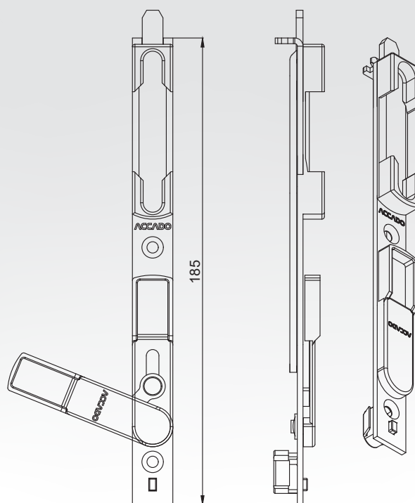
Lever Shoot Bolt, Bottom
