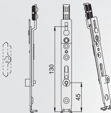
Extension Piece, 90°
